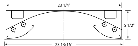
End View: 2 x 4 Side Direct/Indirect with T5 Lamps
